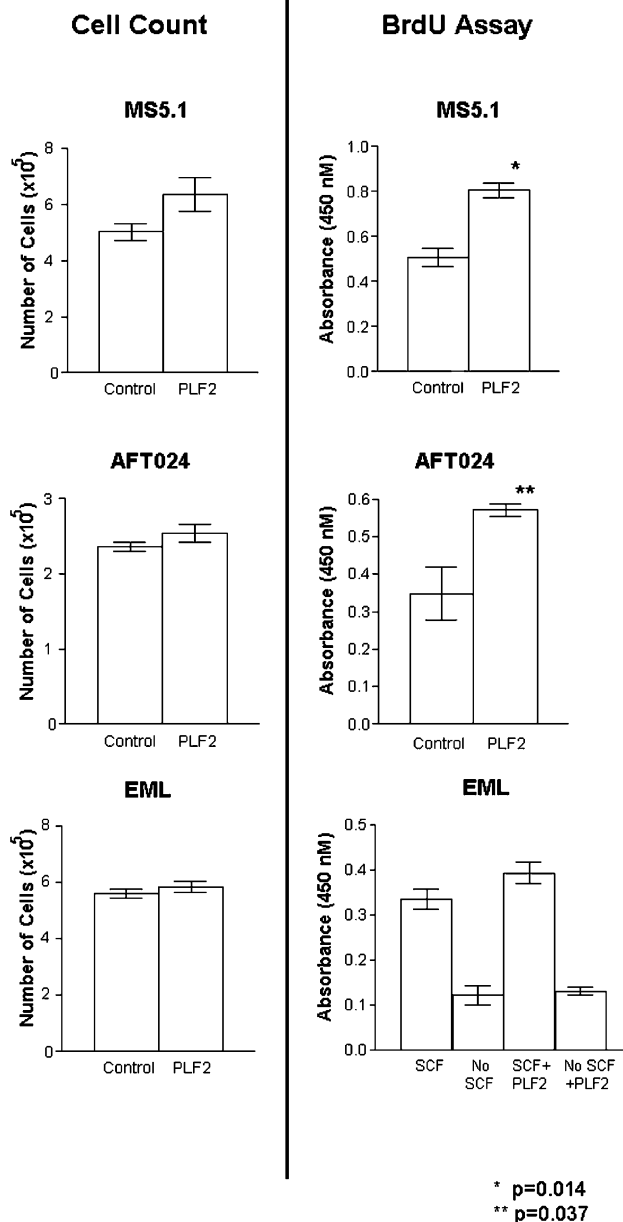
Fig. 5. Effects of PLF2 on cell proliferation. Viable cell count (A) and BrdU assays (B) were performed 96 h after administration of 100 nM PLF2. The controls were cells without PLF2 treatment. Results are shown as means with S.E.M. indicated by the error bars.
